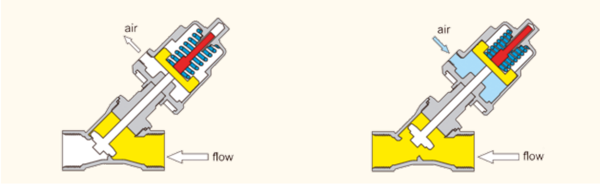
Valve Closed
